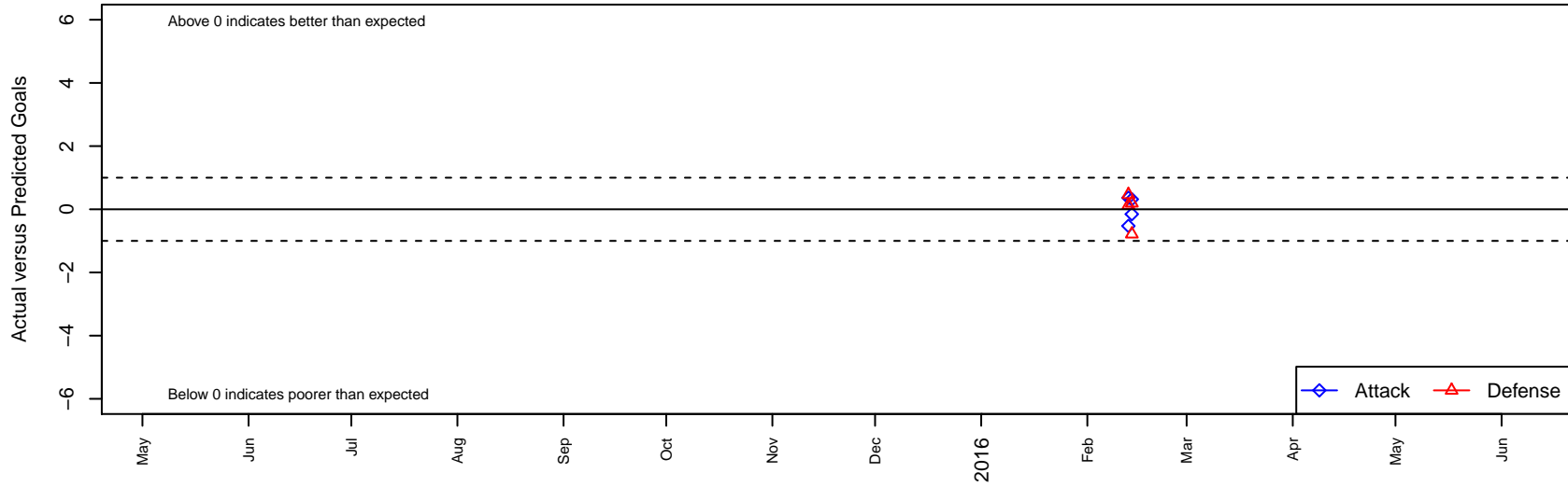
Classic FC Terminators B98 Dots are actual minus expected GF (blue circles) and GA (red triangles). Blue line is smoothed change in attack strength. Red is smoothed change in defense strength.
